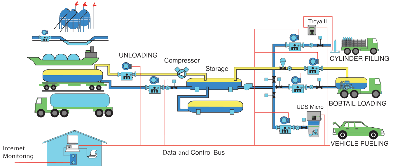
Measurement of every flow in the facility guards against product loss.
